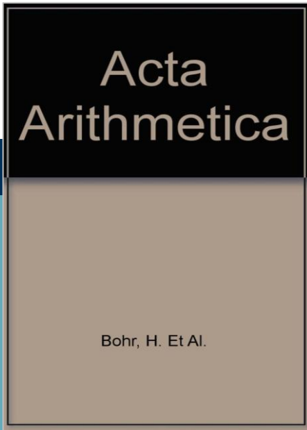
Acta Arithmetica
