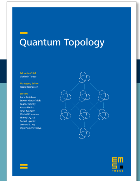
Quantum Topology
